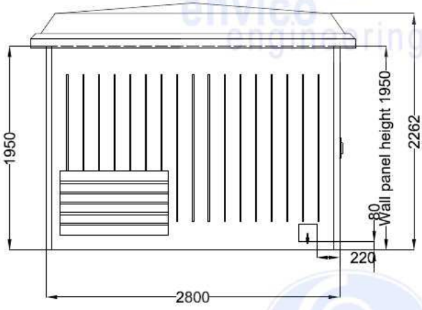
External Elevation Wall 2
