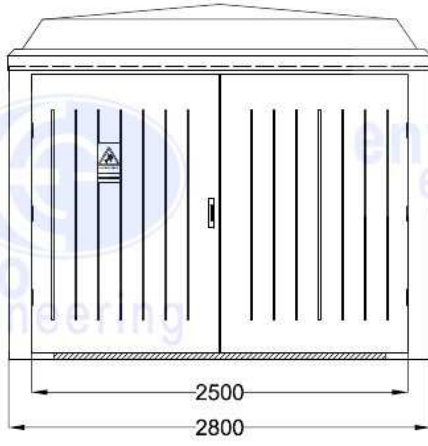
External Elevation Wall 1
