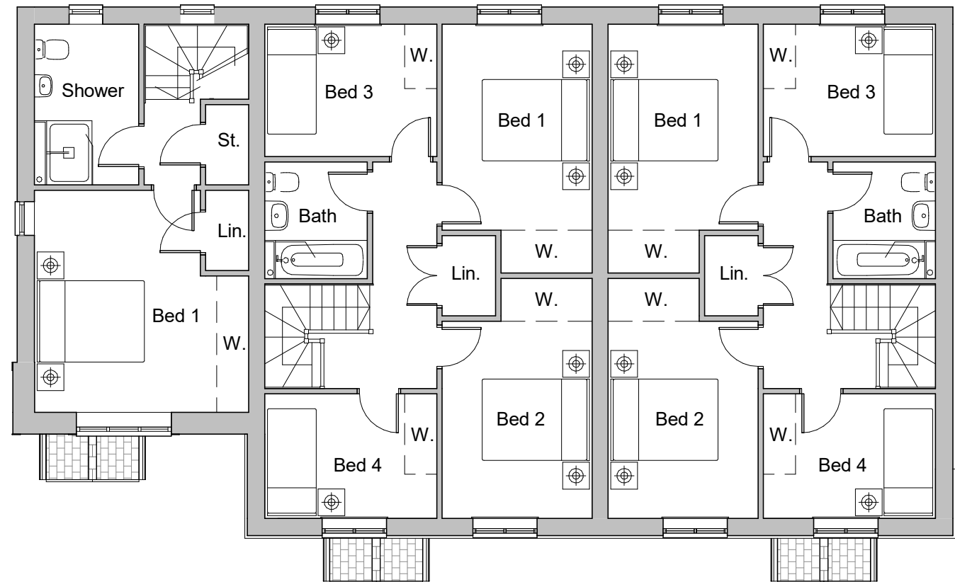
2 0.01 First Floor 1 : 100
