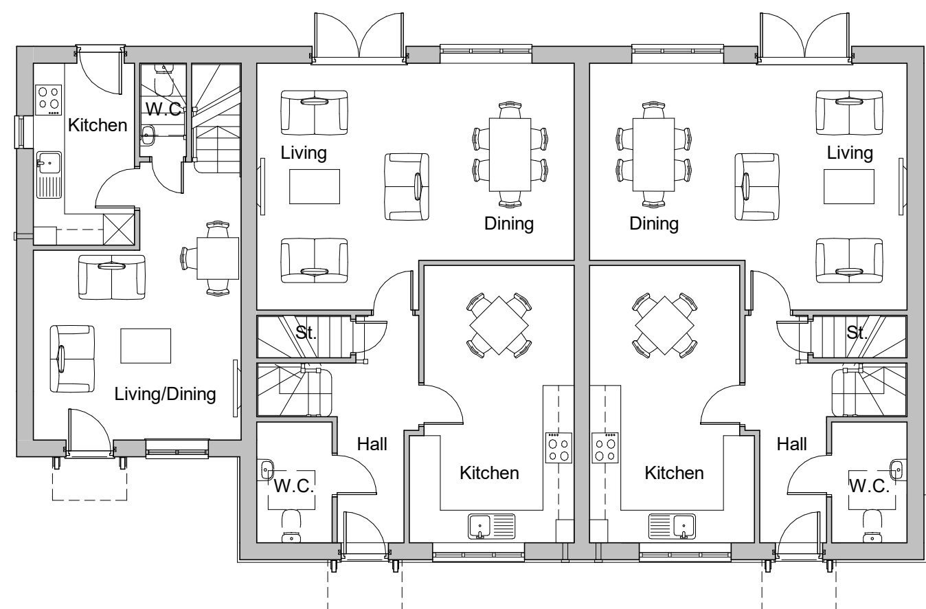
1 0.00 Ground Floor 1 : 100
