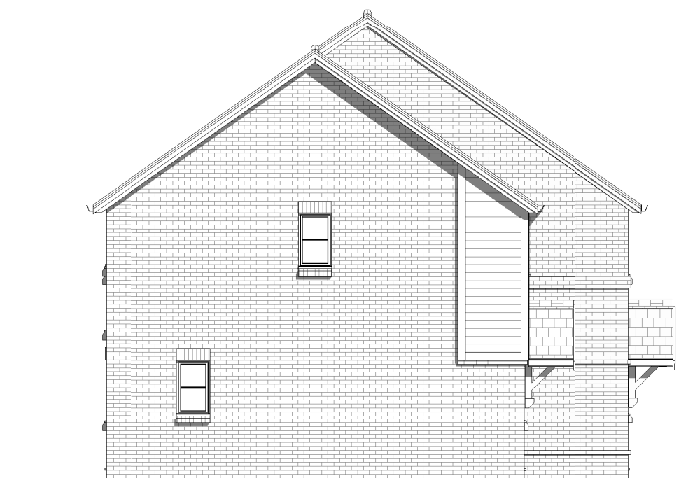
7 Side Elevation - Left 1 : 100
