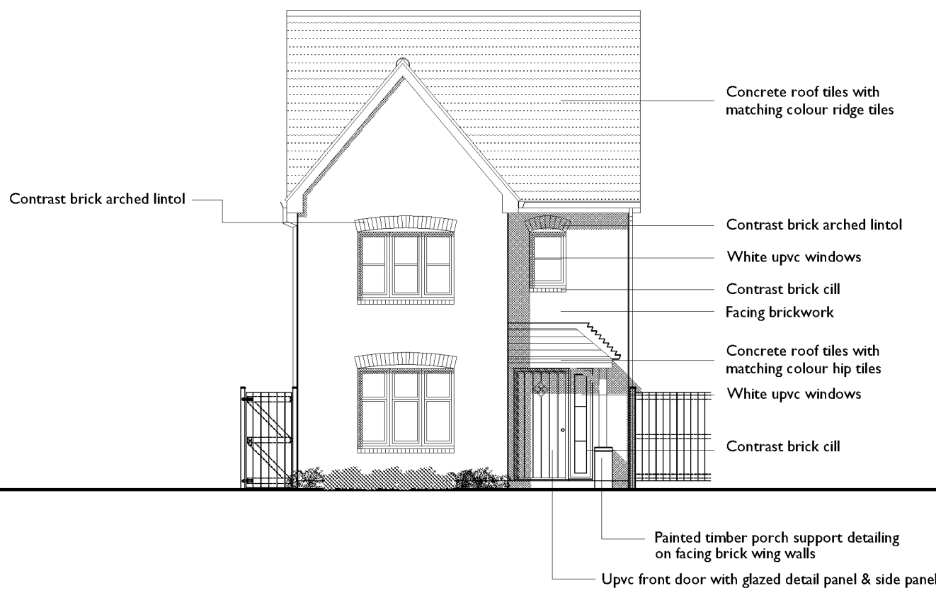
Front Elevation Wall areas left clear to elevations are in facing brickwork
