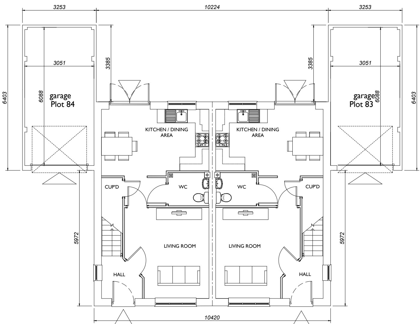
Plot 84 Plot 83 Ground Floor Plan
