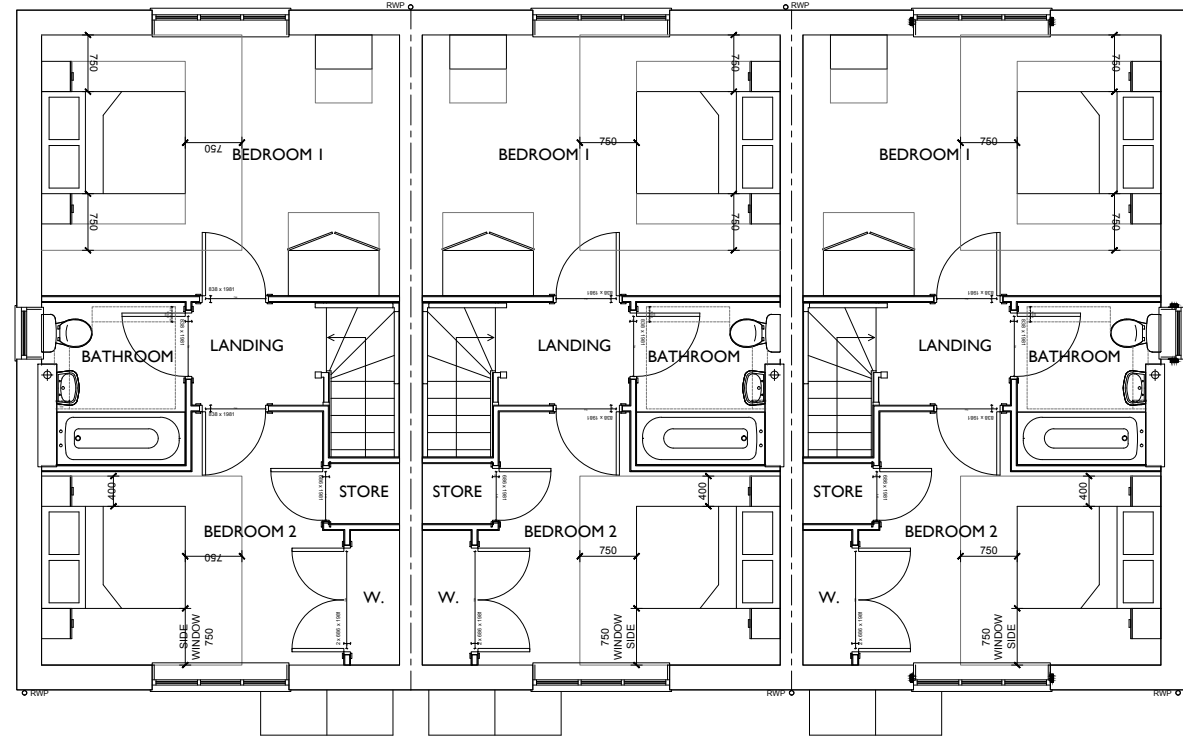
Plot 66 Plot 65 Plot 64 First Floor Plan
