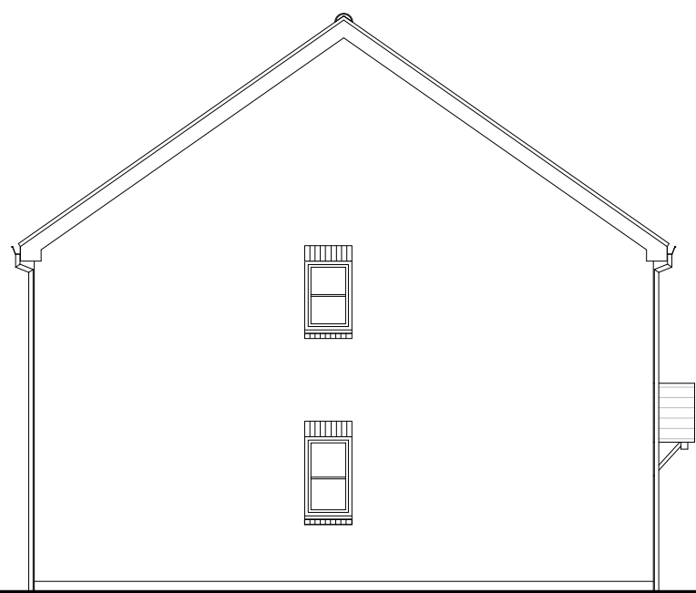
Plot 66 Side Elevation
