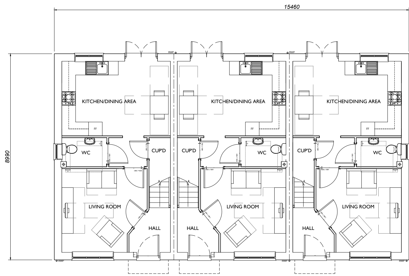
Plot 66 Plot 65 Plot 64 Ground Floor Plan
