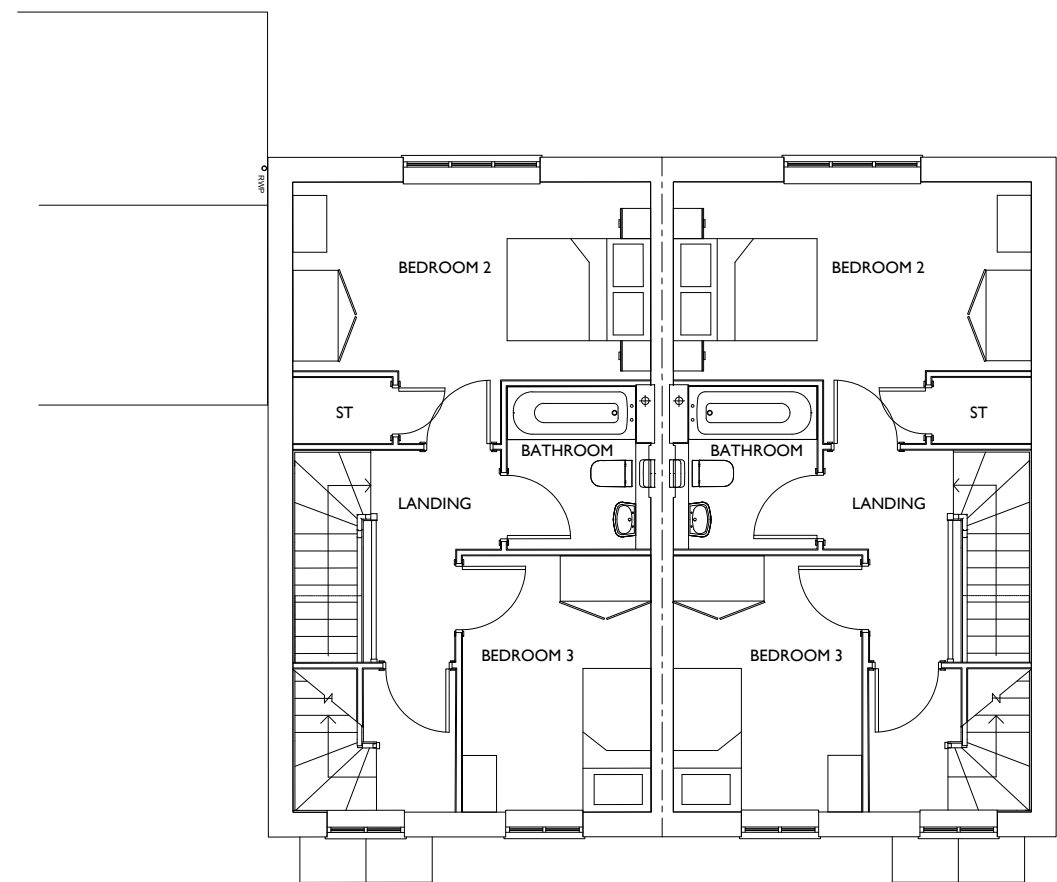
Plot 12 Plot 13 First Floor Plan
