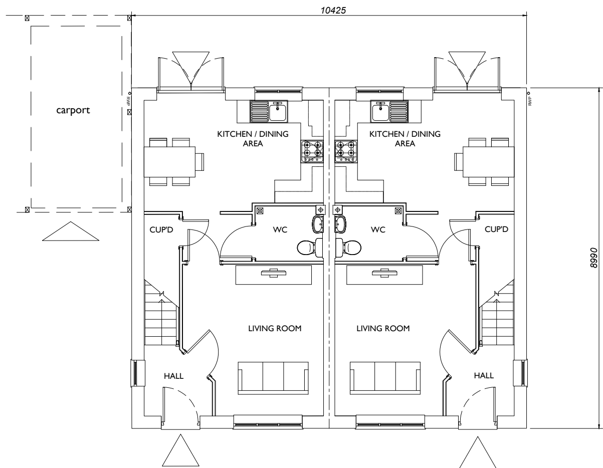
Plot 12 Plot 13 Ground Floor Plan
