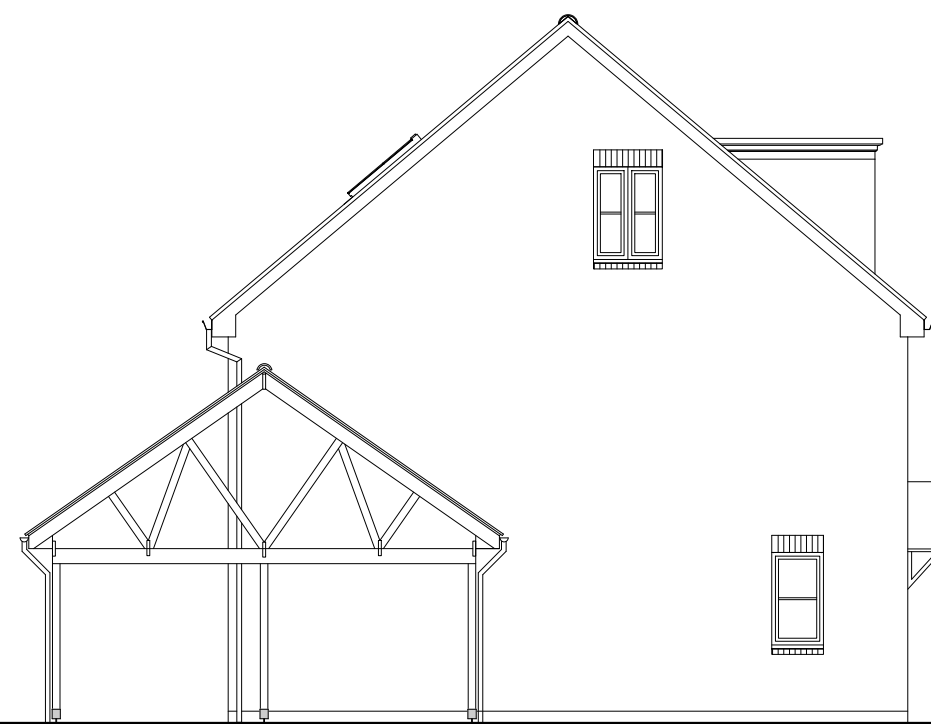
Plot 12 Side Elevation
