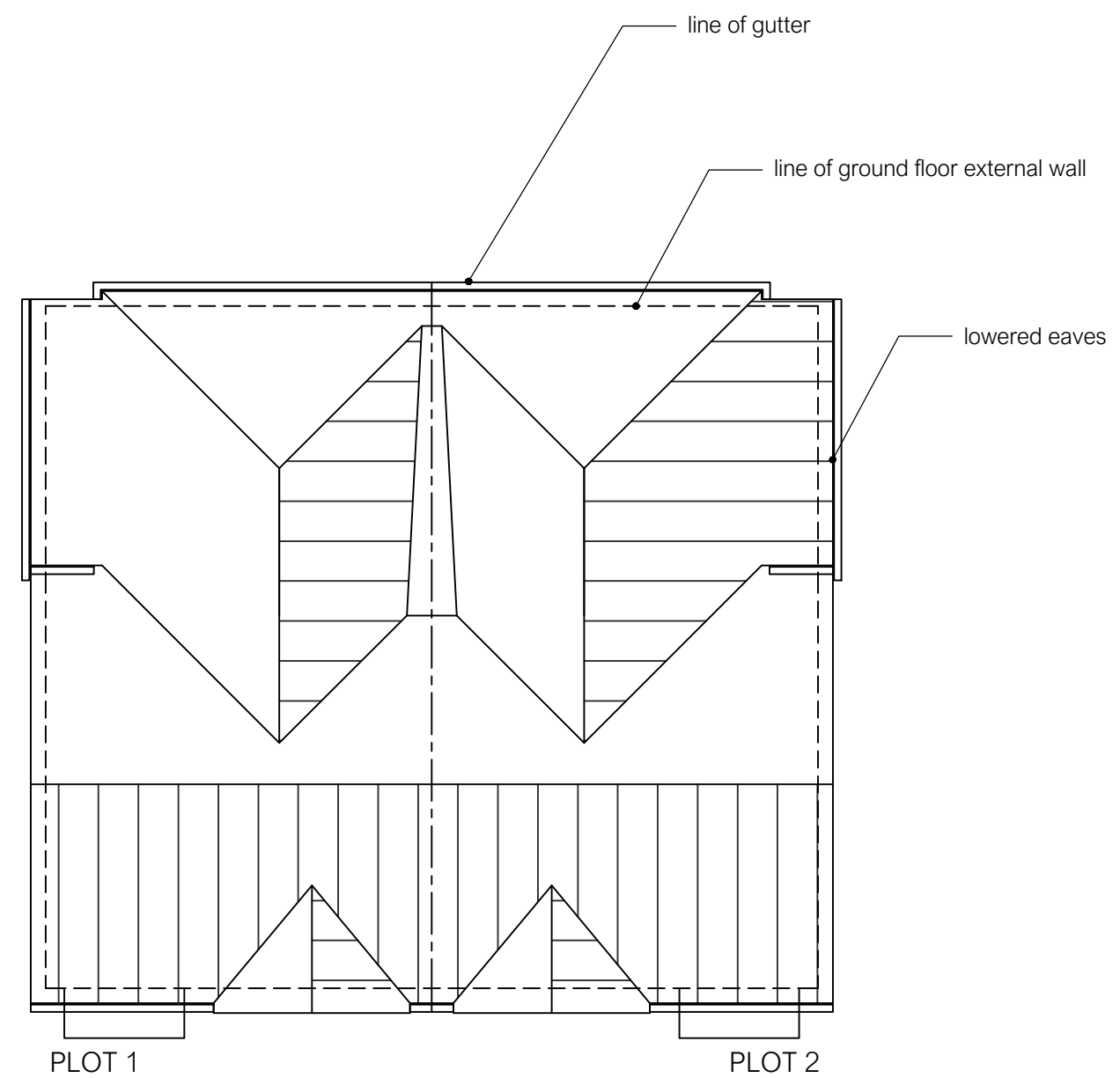
roof plan 1:100
