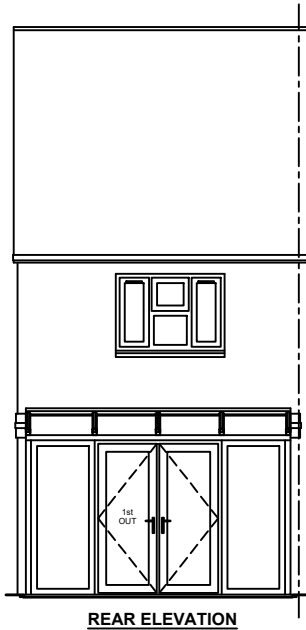
REAR ELEVATION
