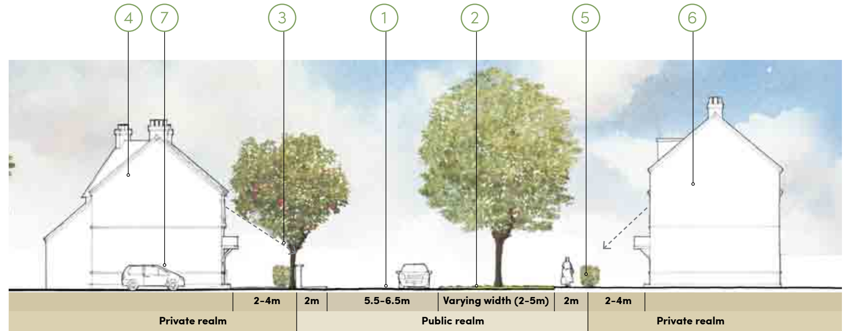
FIGURE 30. Typical section through the Village Street (Residential Spine Road)
