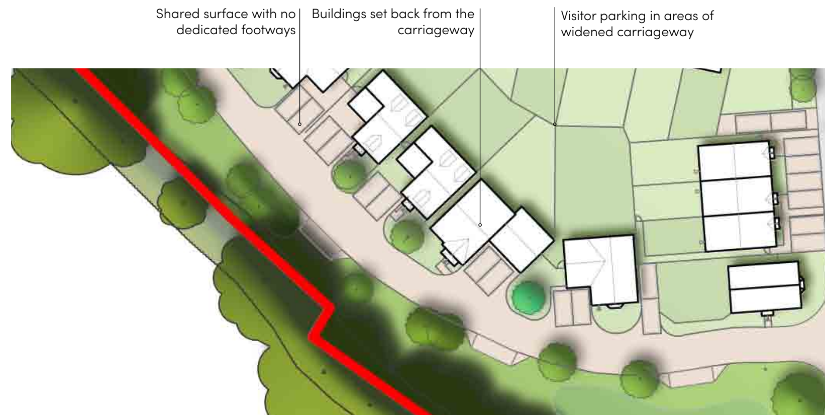
FIGURE 37. Illustration showing the a typical layout of a Residential Street
