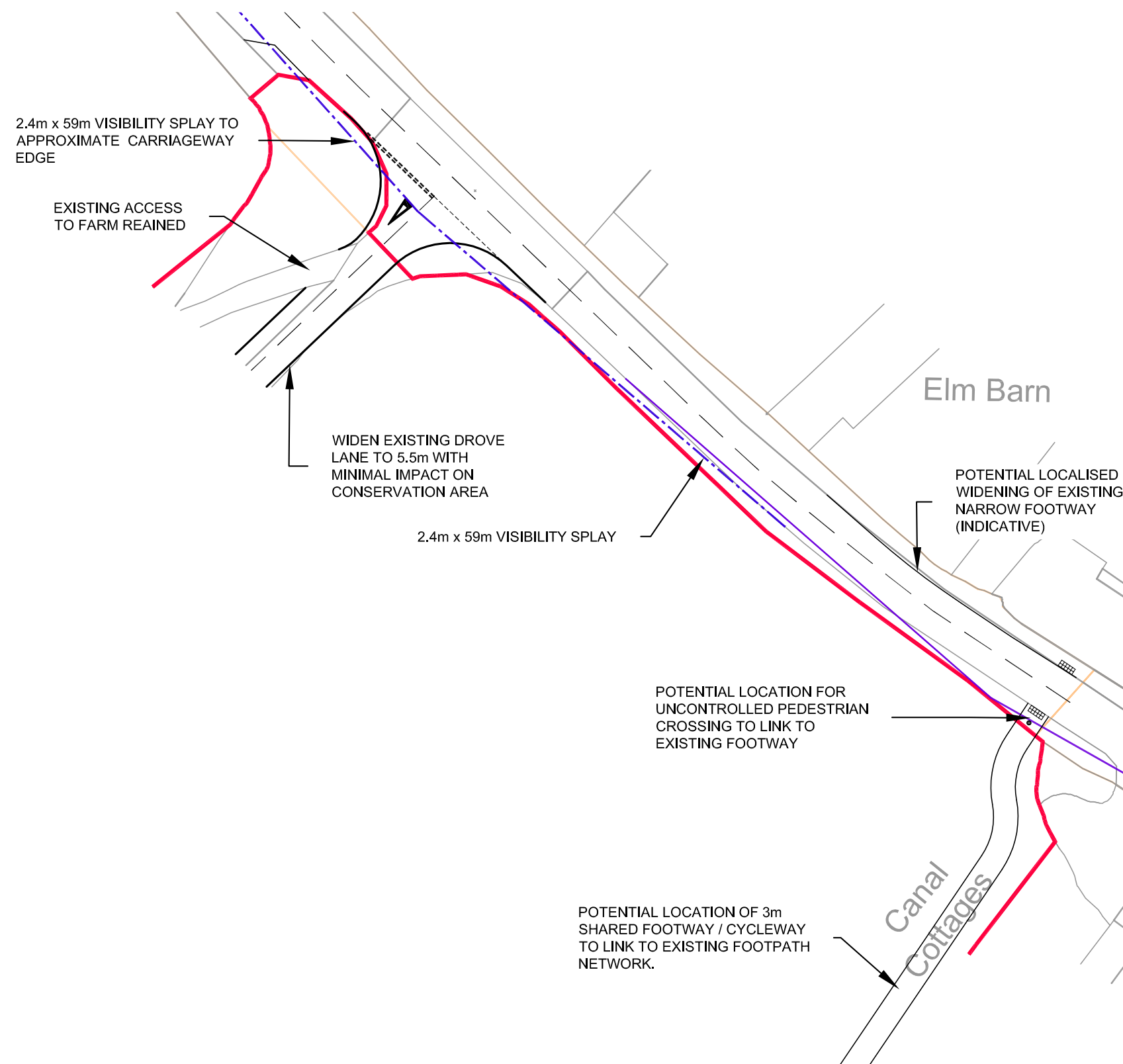
FIGURE 81. Proposed access arrangements for the site
