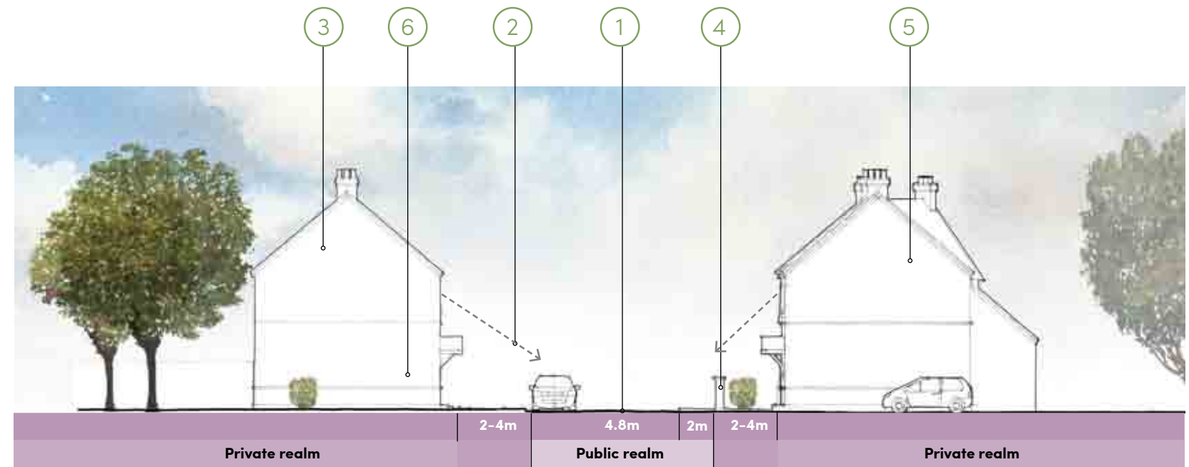
FIGURE 34. Typical section through the Residential Street
