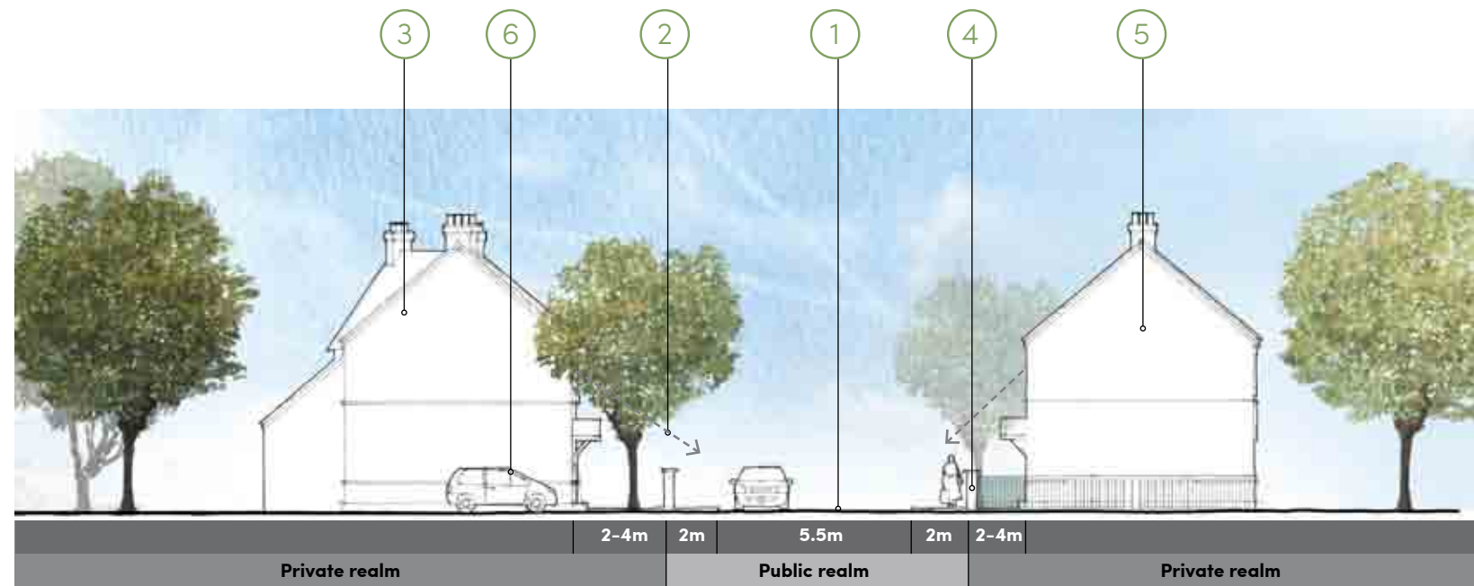
FIGURE 32. Typical section through the Residential Street
