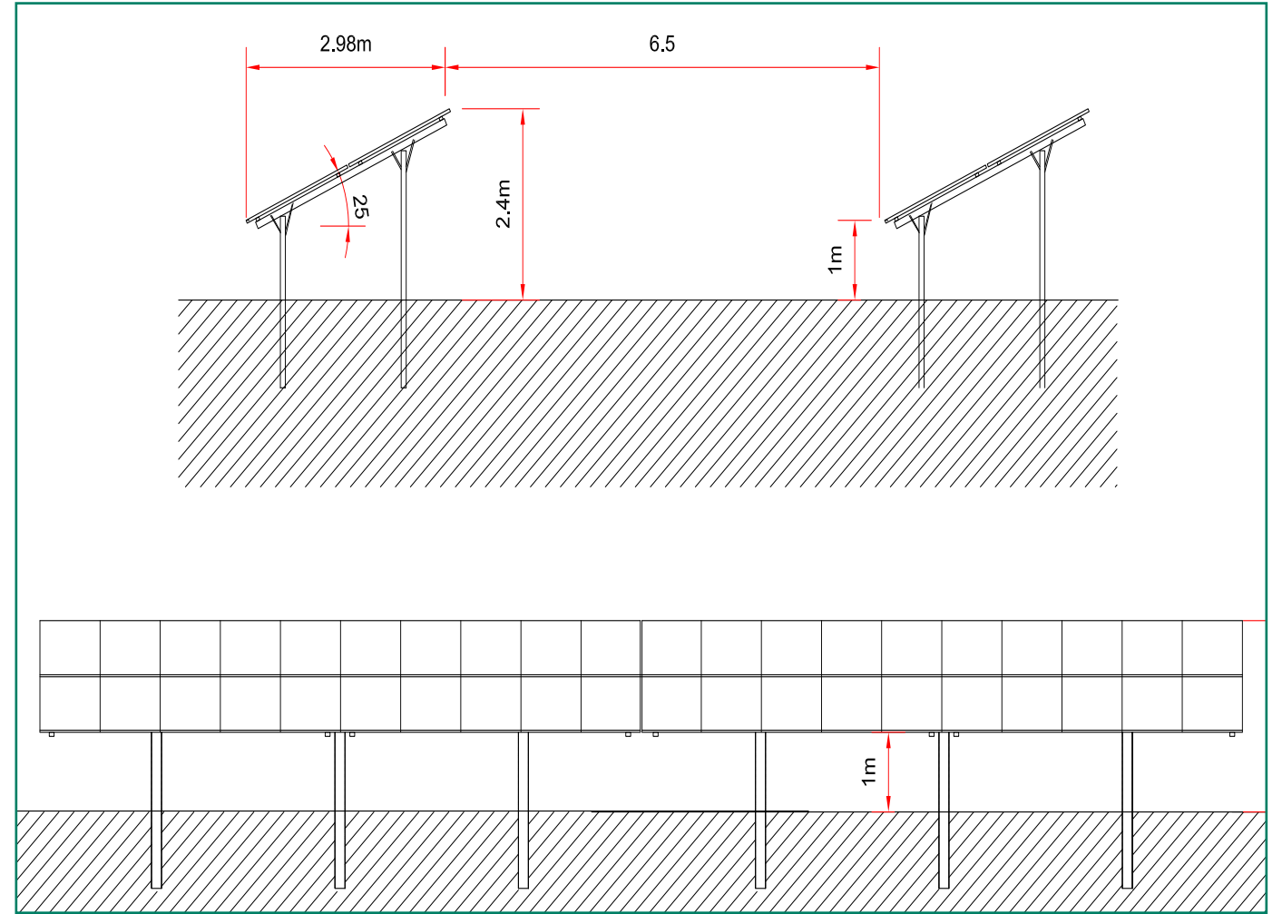
Panel Detail B (not to standard scale)
