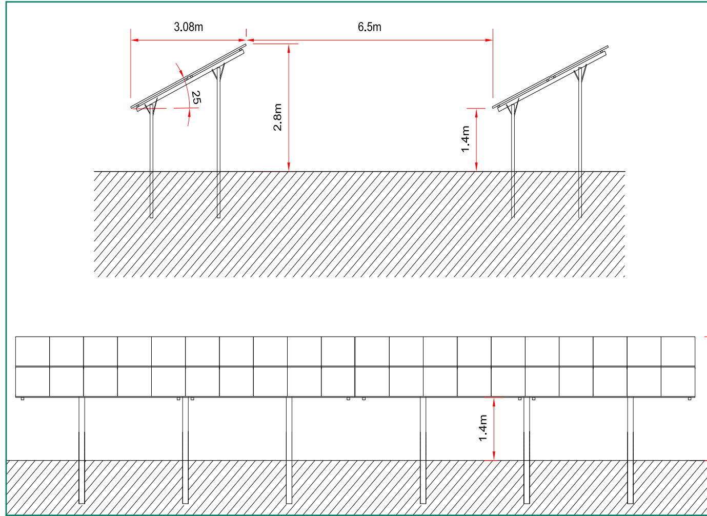
Panel Detail A (not to standard scale)
