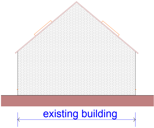
East Elevation
