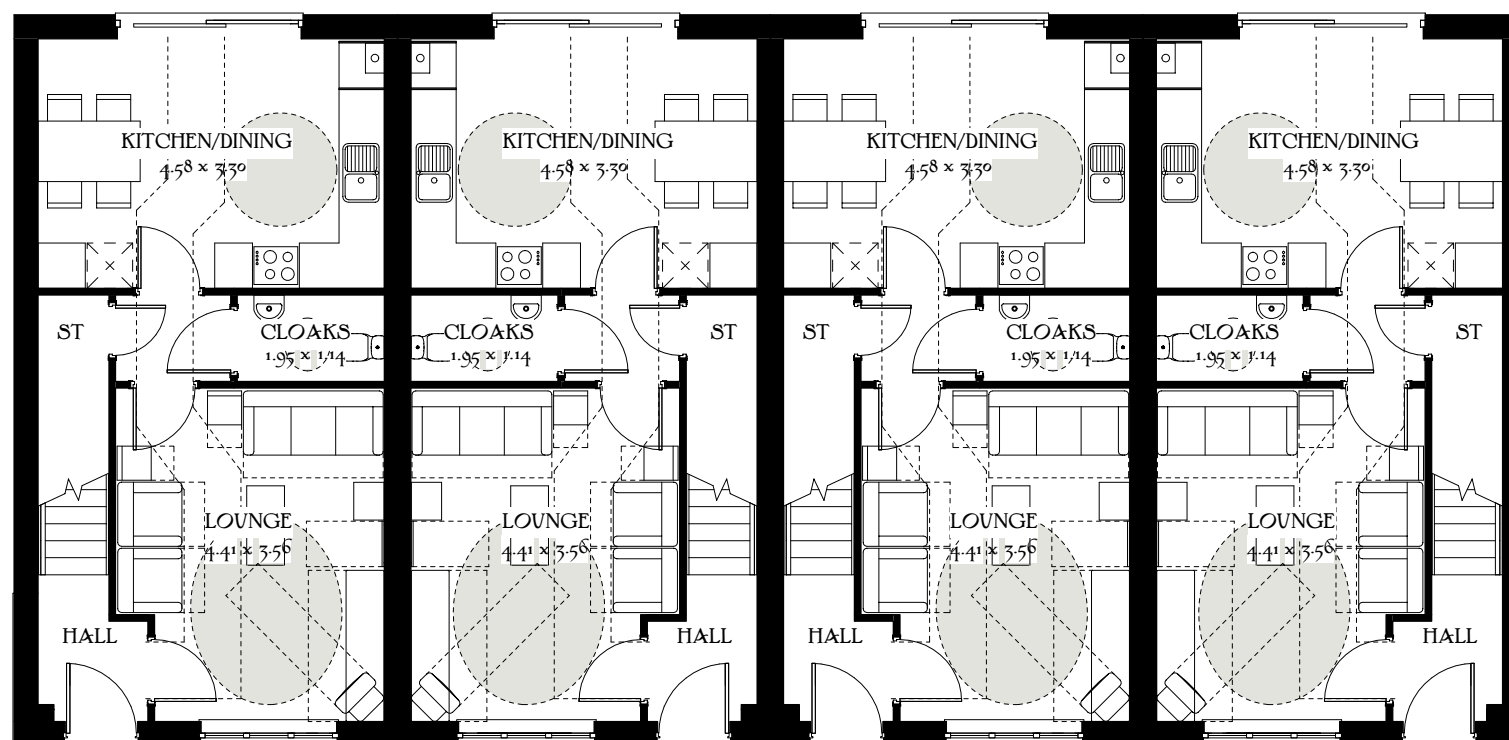
Ground Floor
