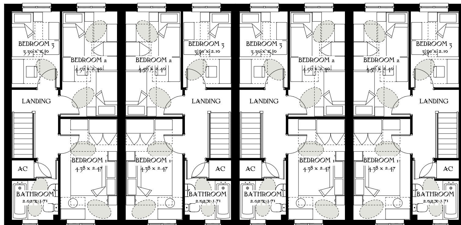
First Floor
