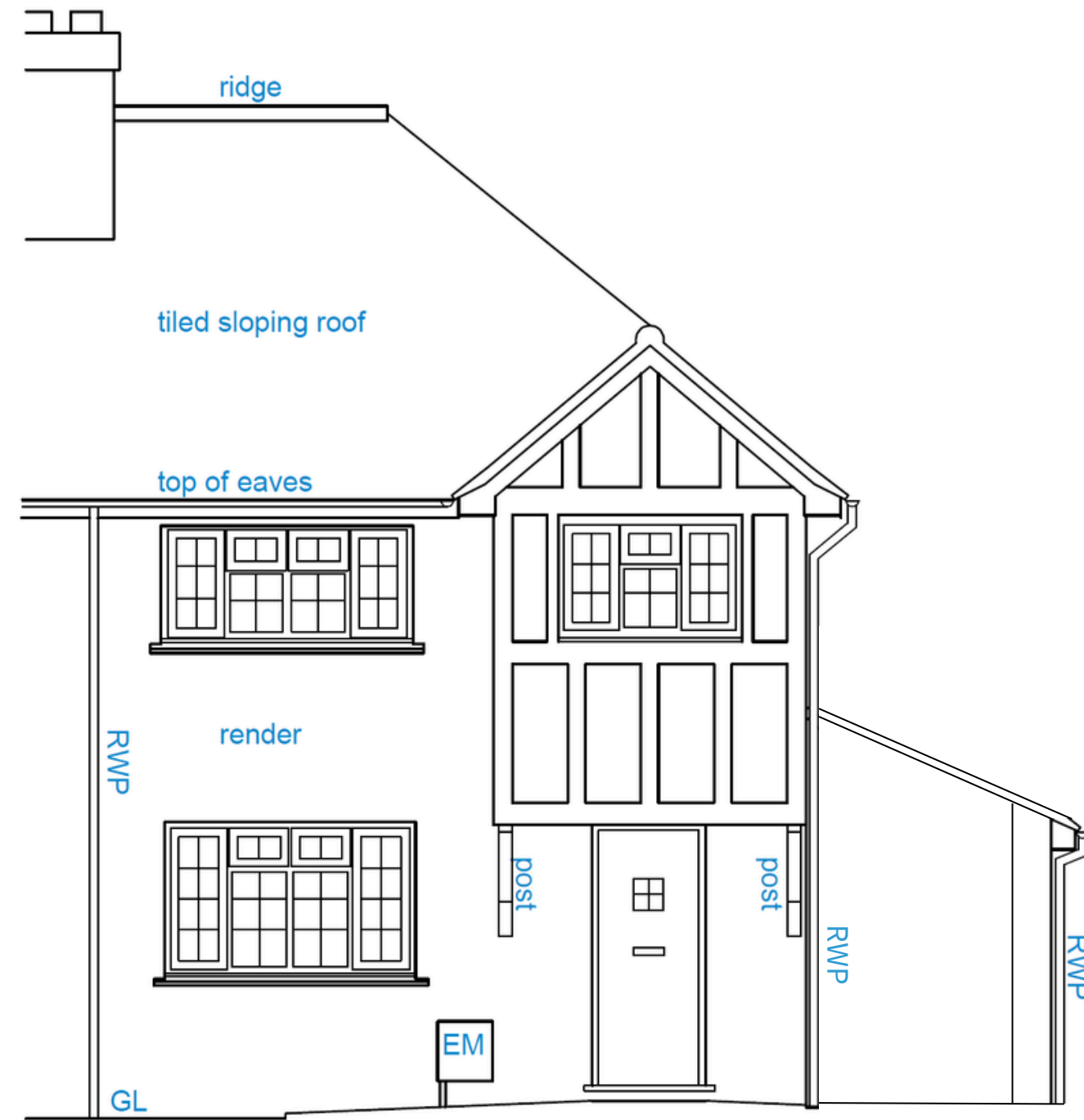
FRONT ELEVATION 1:100
