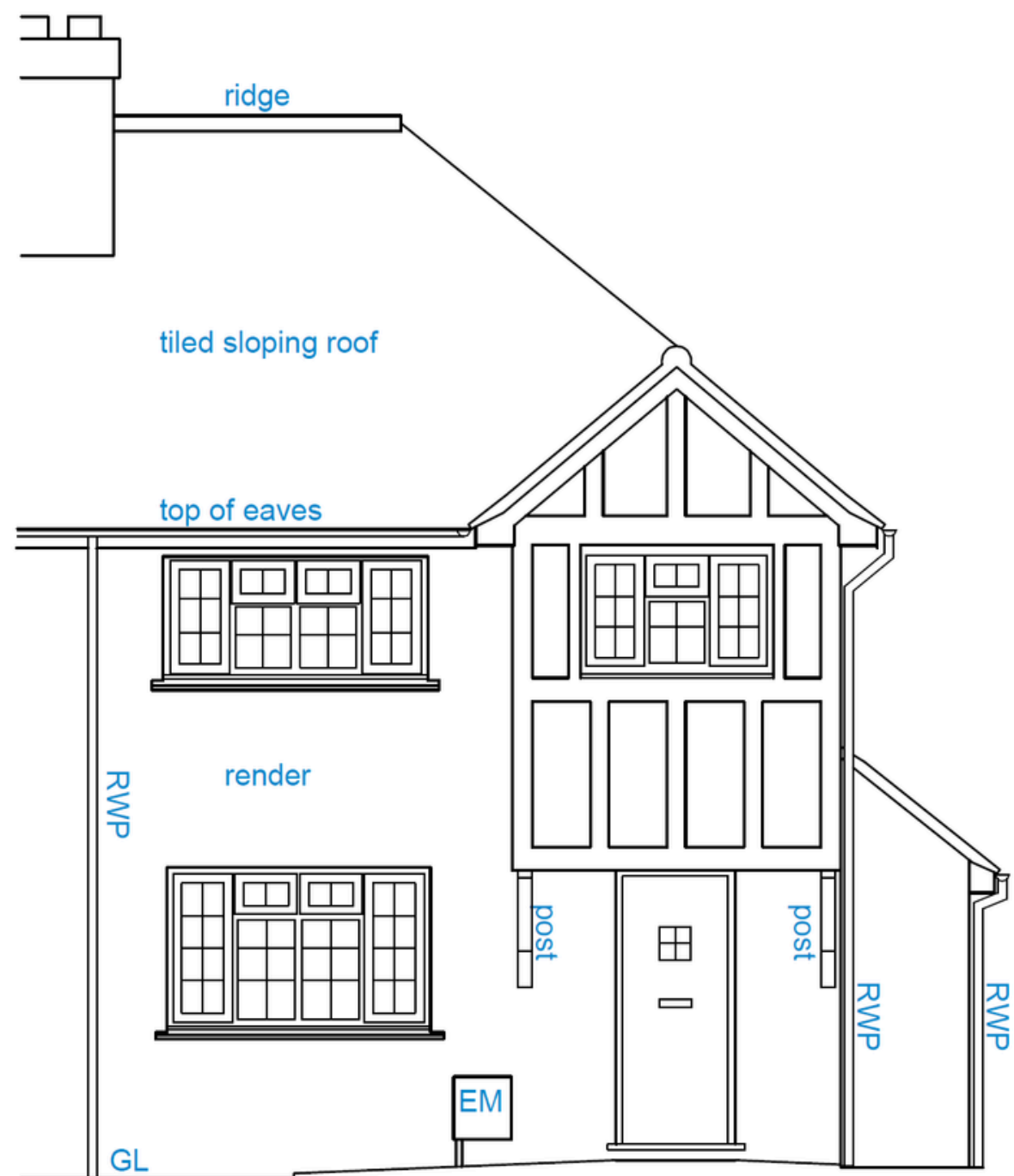
FRONT ELEVATION 1:100
