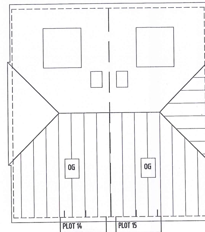
ROOF PLAN
