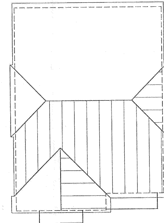
ROOF PLAN
