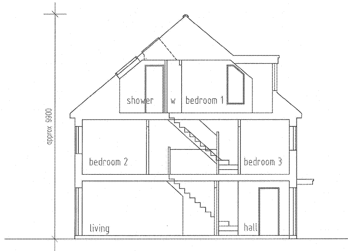
TYPICAL SECTION PLOTS 9-10
