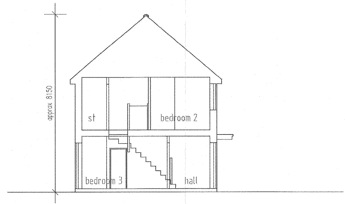
TYPICAL SECTION PLOT 11
