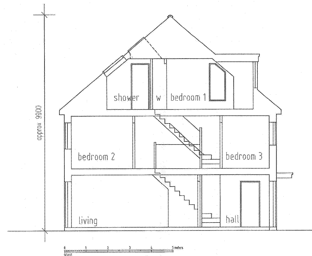
TYPICAL SECTION PLOTS 6-7
