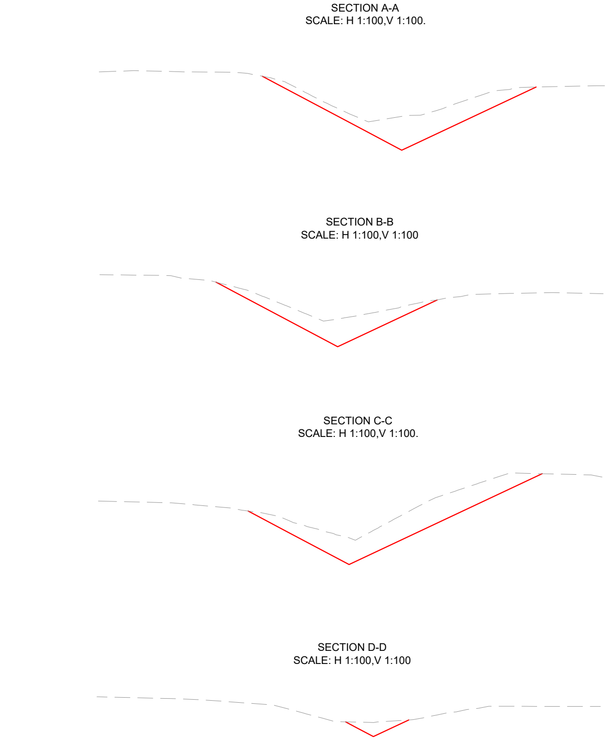
DITCH SECTIONS 1:100
