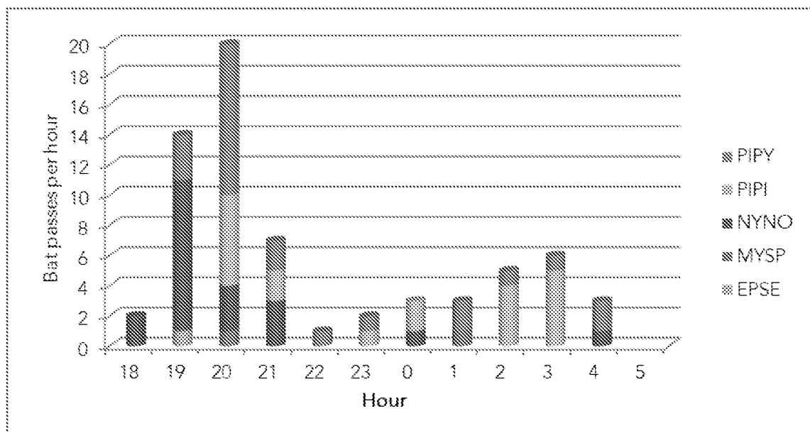
Figure 3.2: Bat passes per hour, 20-24/08/2019, south-west
