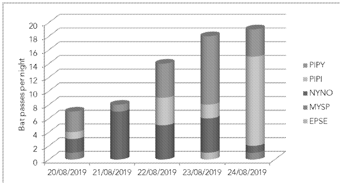
Figure 3.1: Bat passes per night, 20-24/08/2019, south-west
