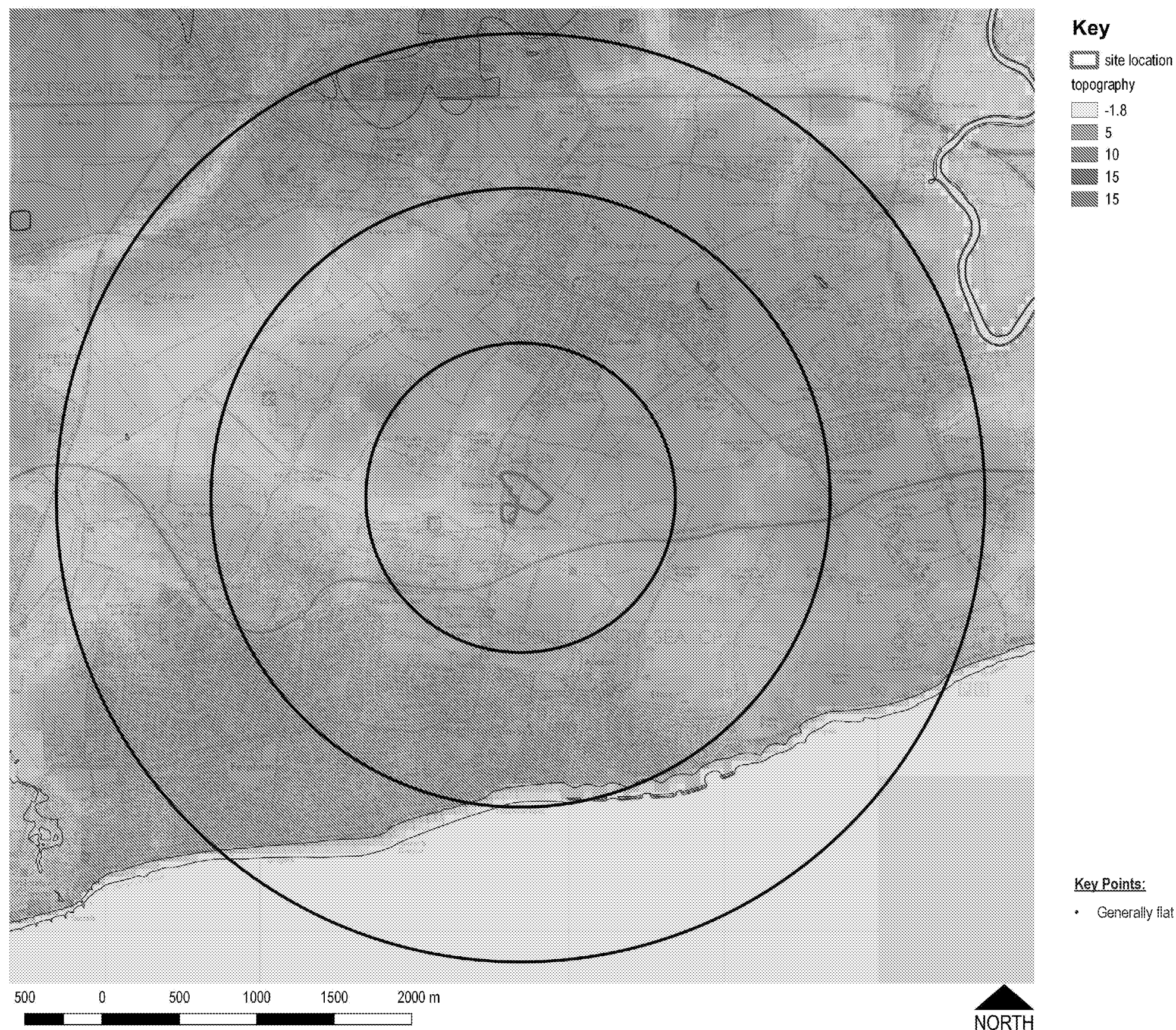
Figure 10 - Topography
