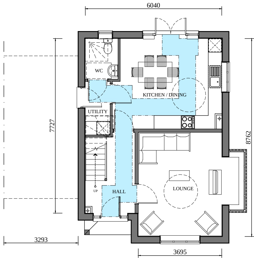
GROUND FLOOR (1:100)
