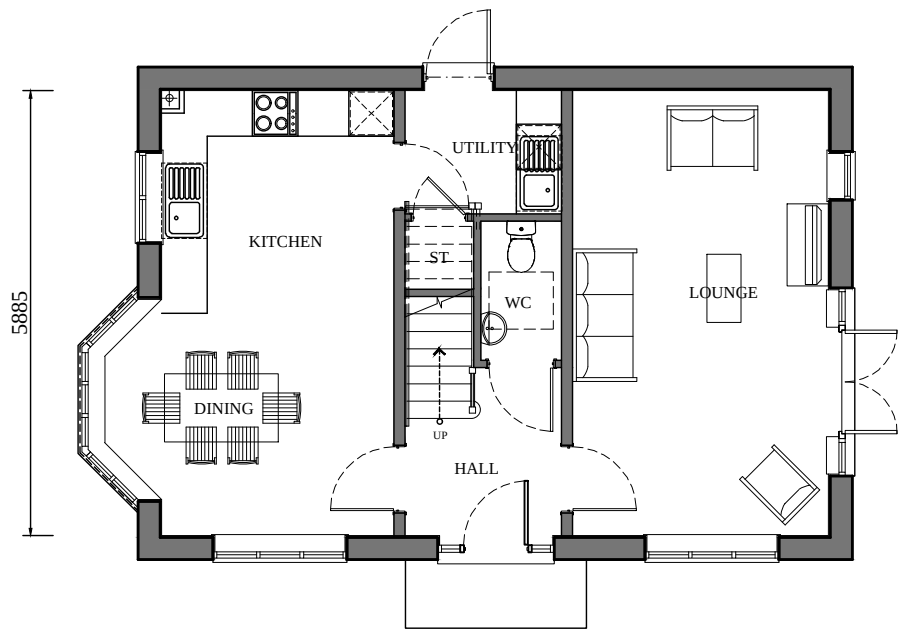
GROUND FLOOR (1:100)
