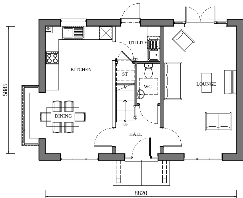
GROUND FLOOR (1:100)
