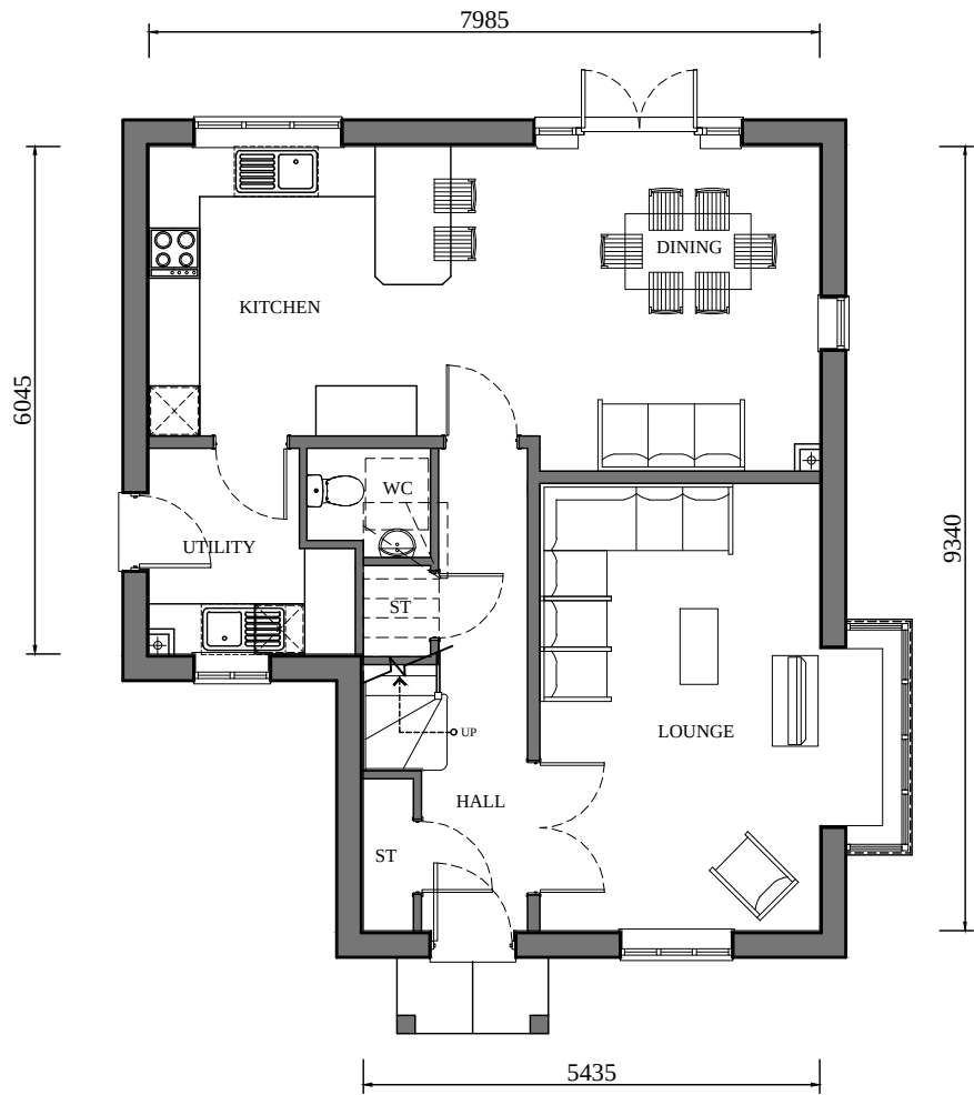
GROUND FLOOR (1:100)
