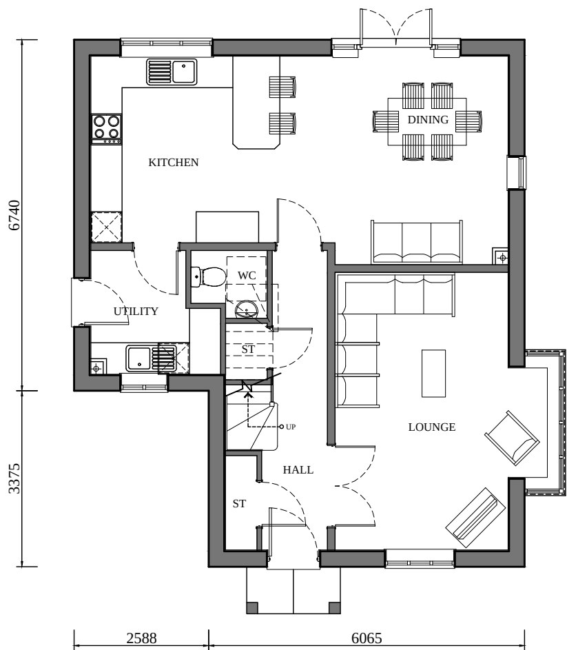
GROUND FLOOR (1:100)
