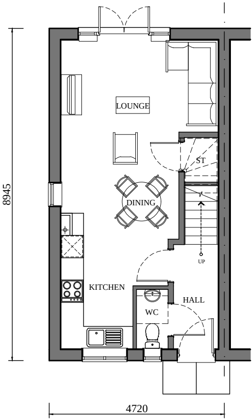
GROUND FLOOR (1:100)
