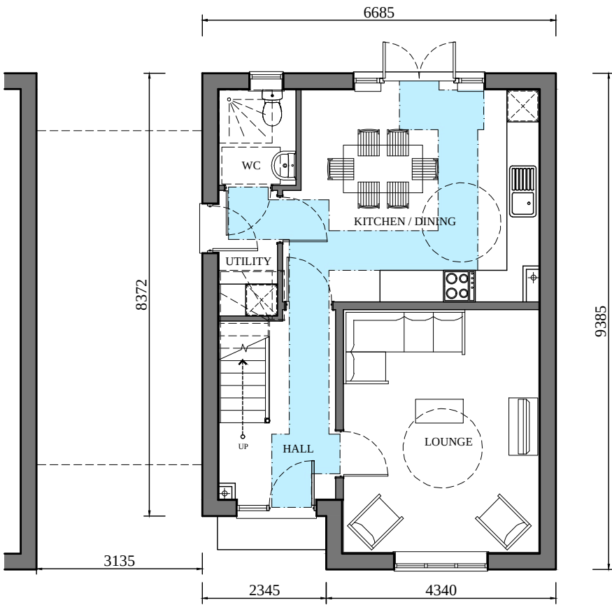
GROUND FLOOR (1:100)
