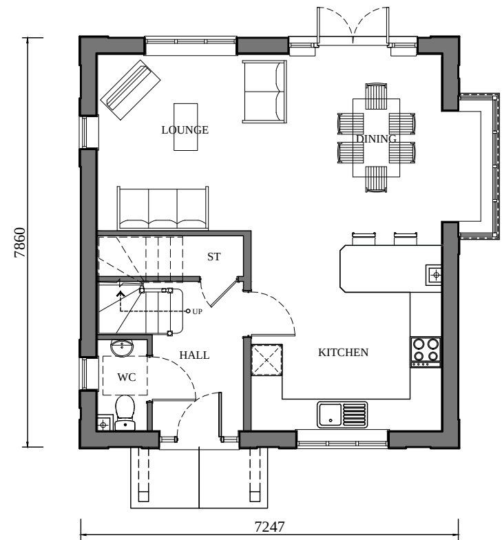
GROUND FLOOR (1:100)
