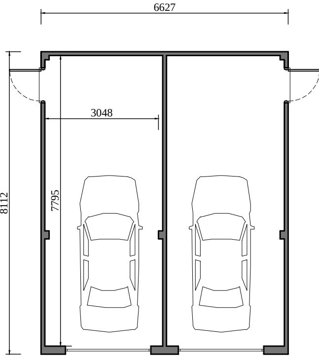
FLOOR PLAN (1:100) DOUBLE GARAGE DETACHED
