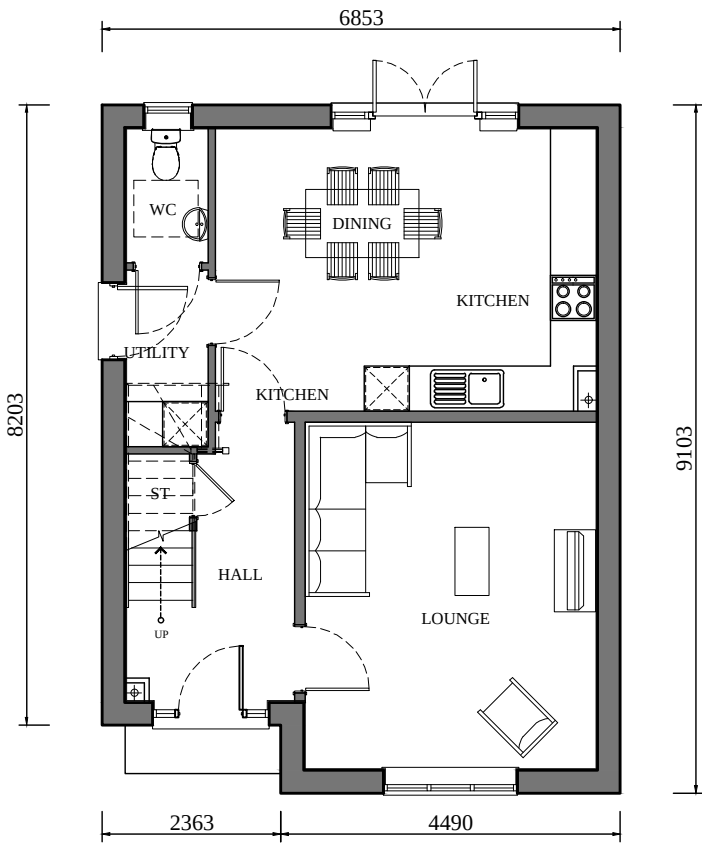
GROUND FLOOR (1:100)
