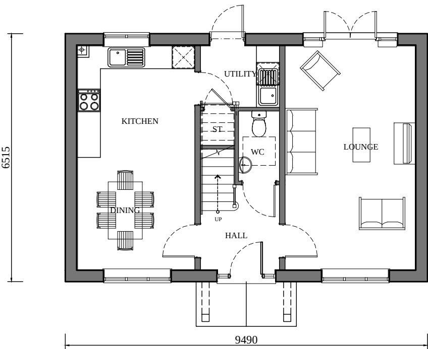
GROUND FLOOR (1:100)
