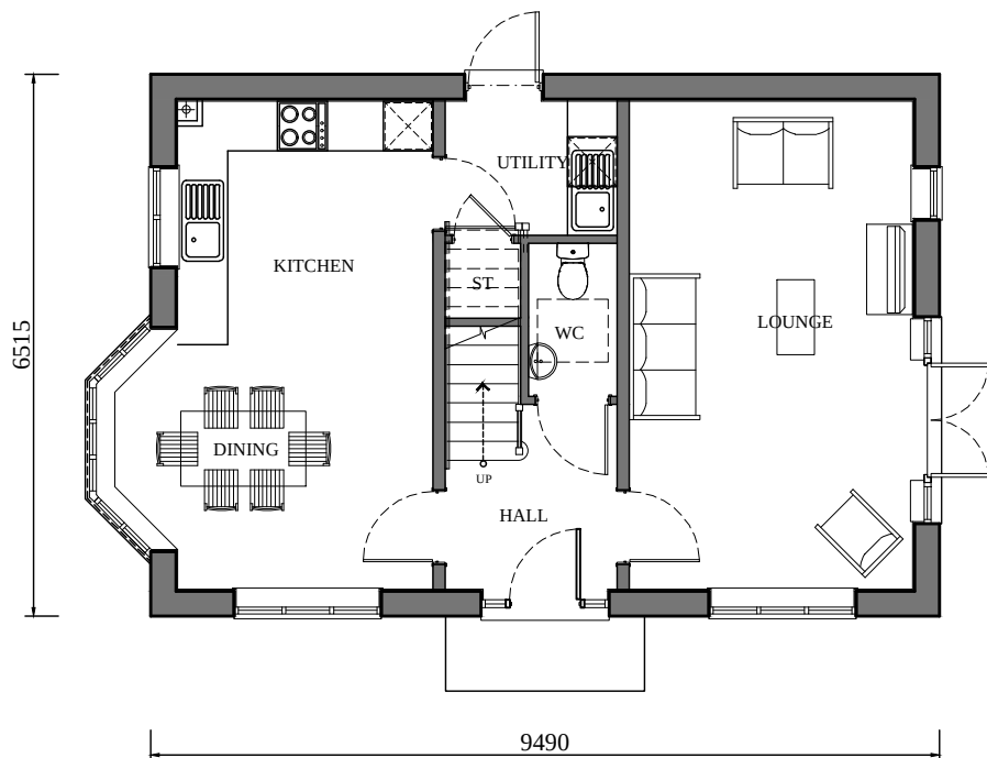
GROUND FLOOR (1:100)
