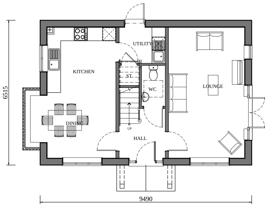
GROUND FLOOR (1:100)
