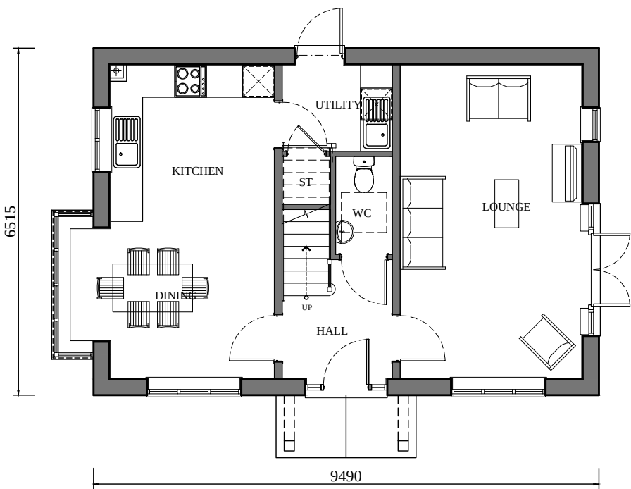
GROUND FLOOR (1:100)
