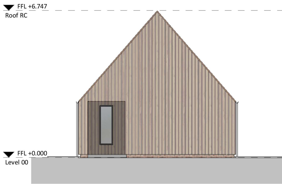
② East Elevation - Remembrance Court 1 : 100
