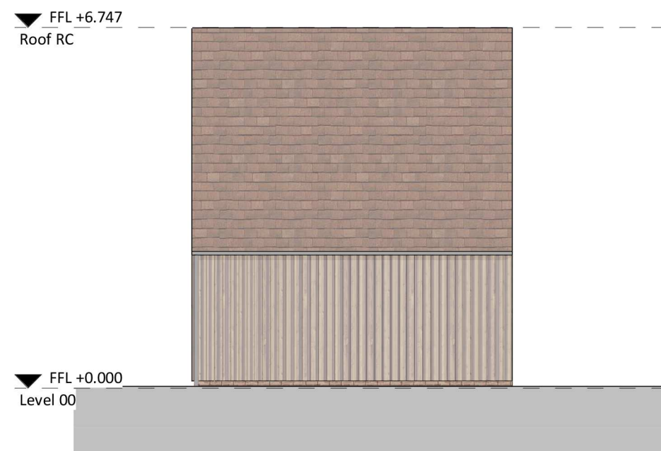
③ South Elevation - Remembrance Court 1 : 100
