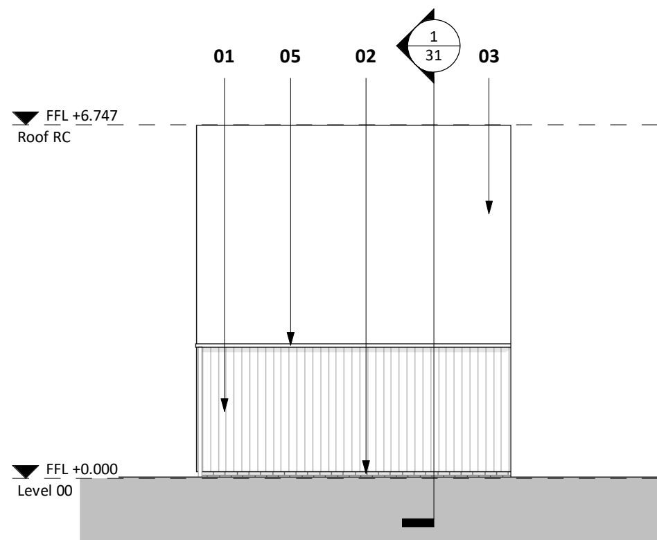
3 South Elevation - Remembrance Court 1 : 100
