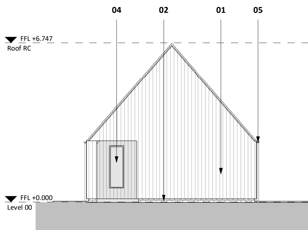
2 East Elevation - Remembrance Court 1 : 100
