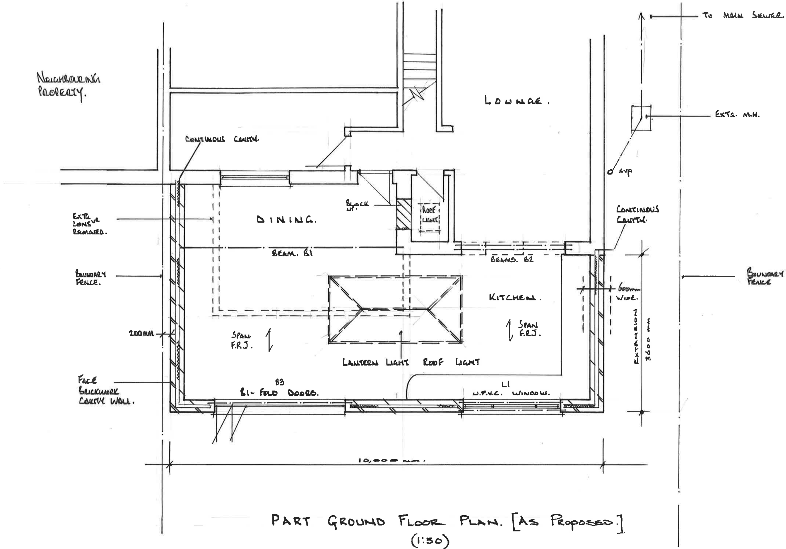
SINGLE STOREY REAR EXTENSION - 32 TACK LEE ROAD, BN18 0HB.
