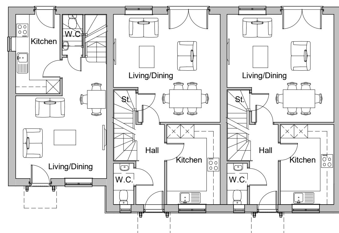
1 0.00 Ground Floor 1 : 100
