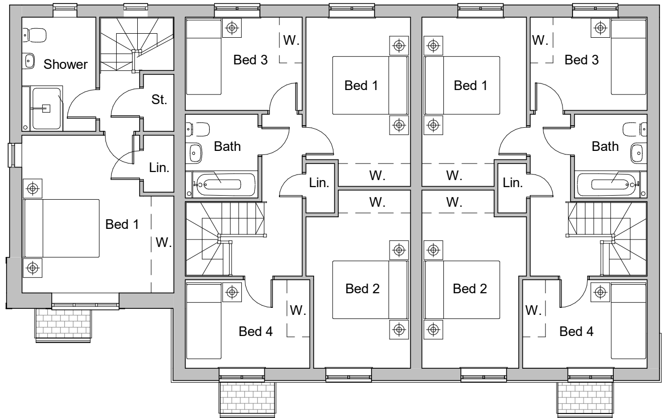
2 0.01 First Floor 1 : 100
