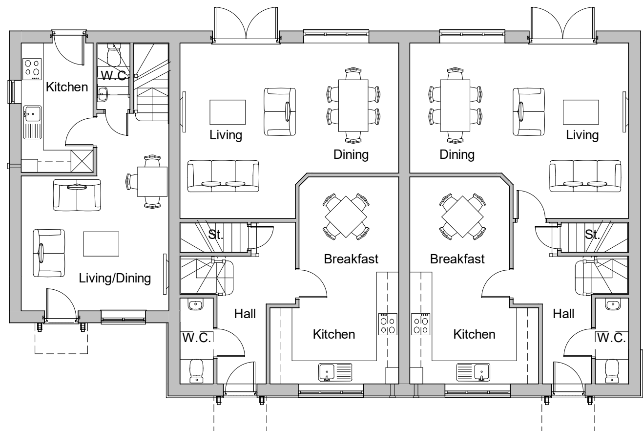
1 0.00 Ground Floor 1 : 100
