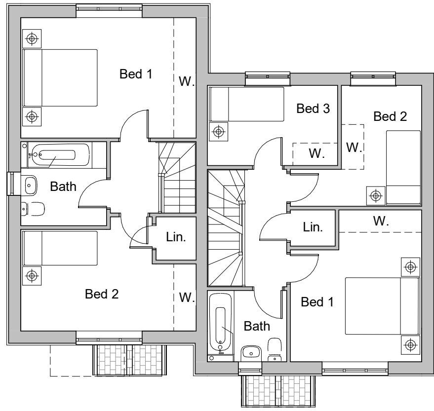
2 0.01 First Floor 1 : 100
