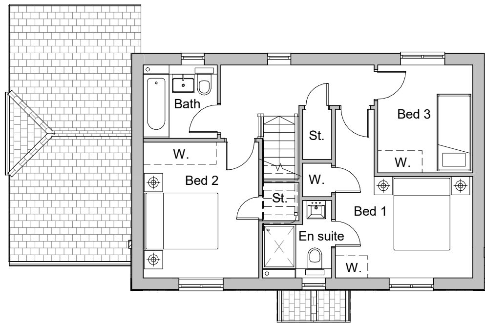
2 0.01 First Floor G3 1 : 100
