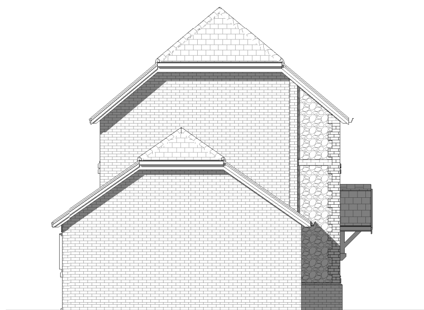
5 Side Elevation - Left G3 1 : 100
