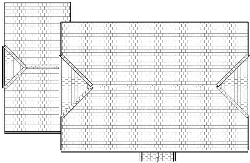
8 0.03 Roof Plan G3 1 : 100
