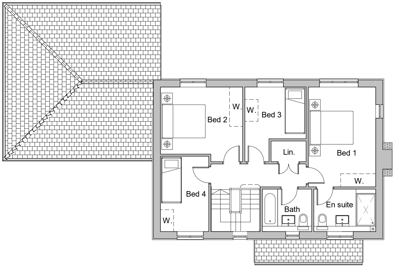
1 0.01 First Floor Plan 1 : 100
