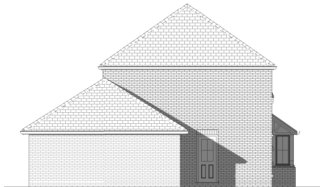
6 Side Elevation - Left A4 1 : 100
