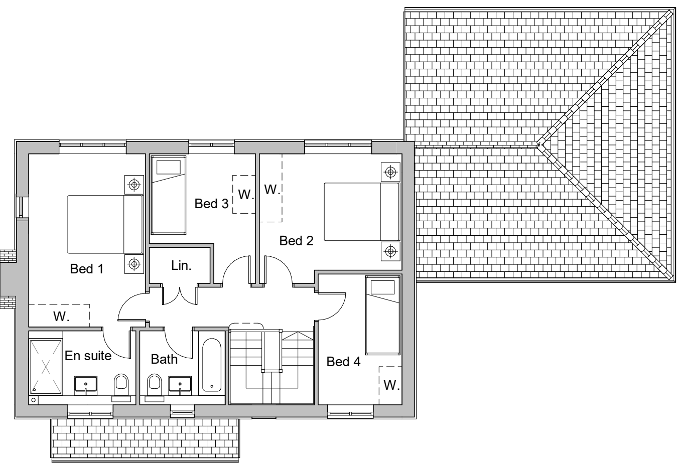
1 0.01 First Floor Plan 1 : 100
