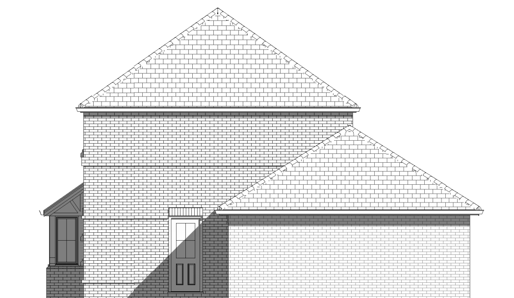
5 Side Elevation- Right A4 1 : 100
