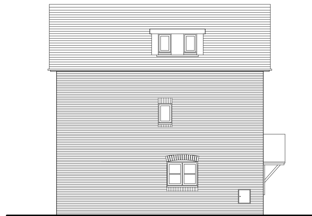
WEST ELEVATION
