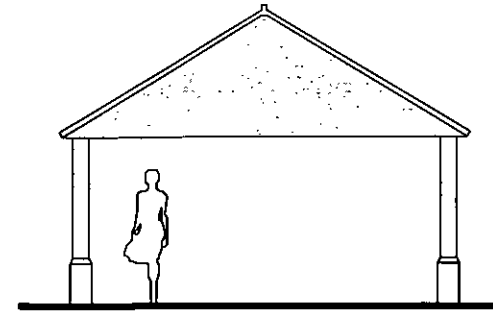
Proposed Side (East) Elevation at 1:100 scale
