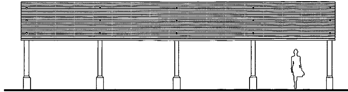
Proposed Front (North) Elevation at 1:100 scale
