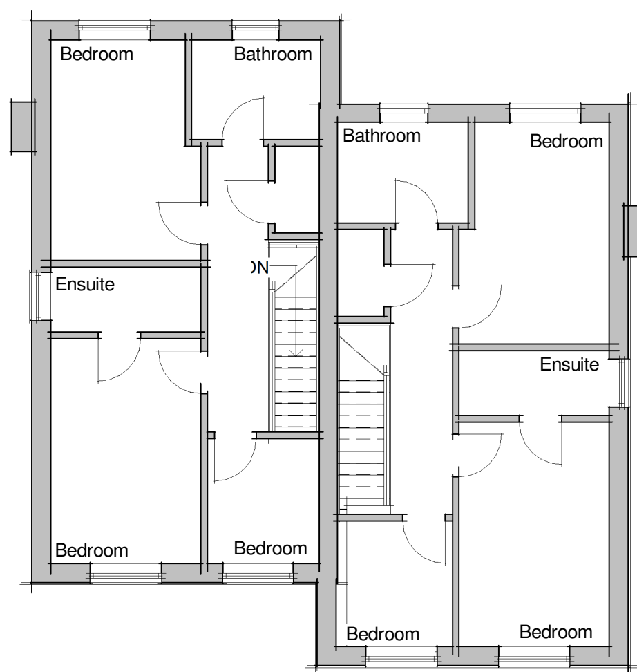
First Floor 1 : 100
