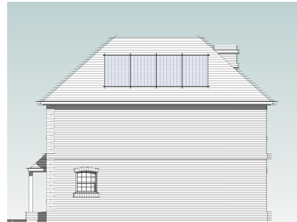
South Elevation 1 : 100
