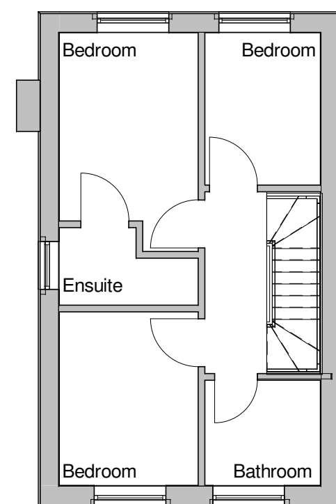
First Floor 1 : 100
