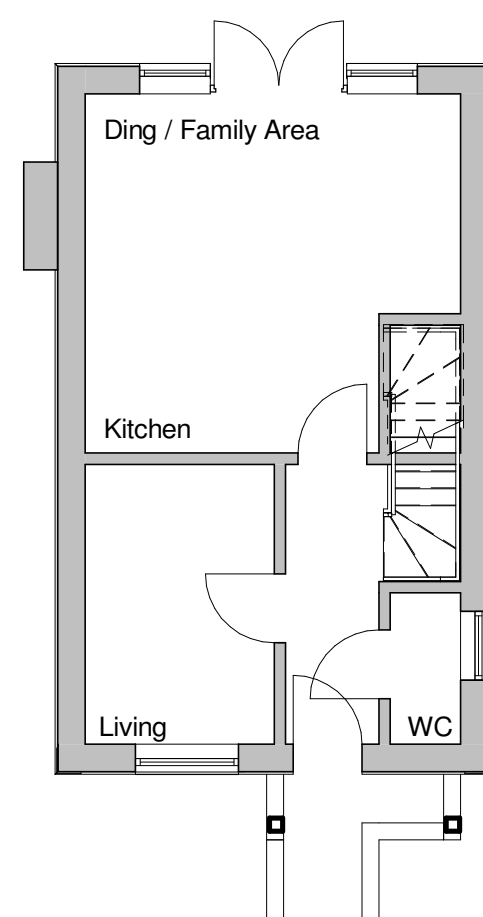
Ground Floor 1 : 100
