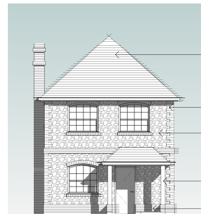
West Elevation 1 : 100
