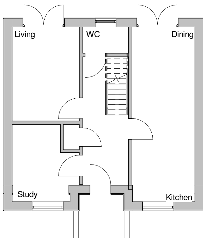
Ground Floor 1 : 100
