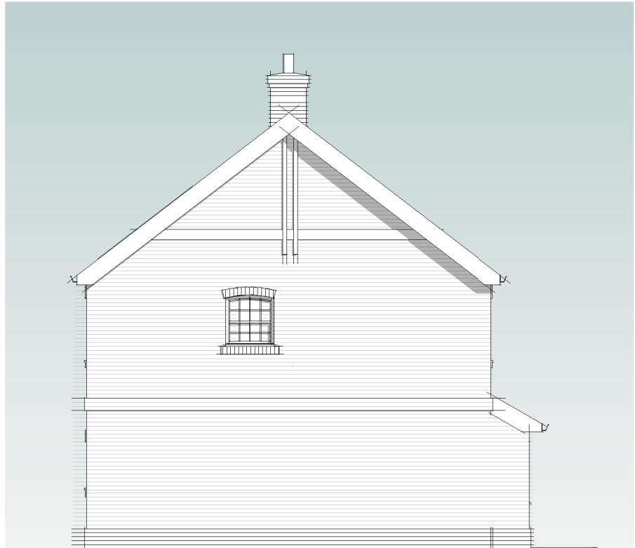
North Elevation 1 : 100
