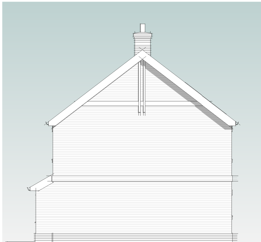
South Elevation 1 : 100
