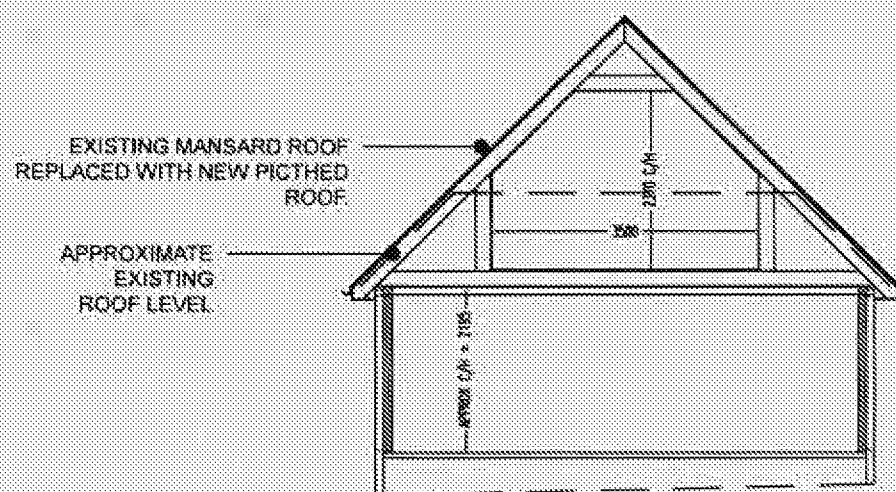
General Section
