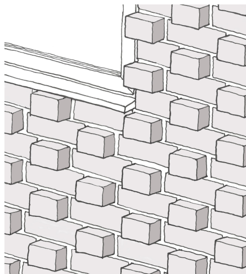
BRICK DETAIL SKETCH Flemish bond with header bricks protruding from face brick
